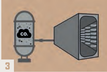
3 Inside curing chamber, water is removed from the concrete to allow the CO 2 to get in and carbonize it, permanently storing the CO 2
