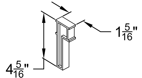
PIN DETAIL
