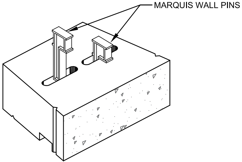
TOP ISOMETRIC
