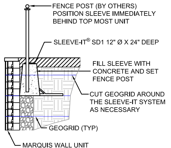
2 1 FENCE POST WITH SLEEVE-IT 1224R
