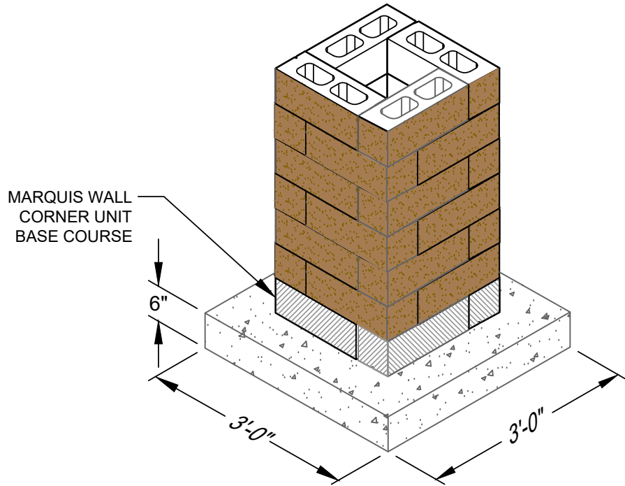
ISOMETRIC VIEW
