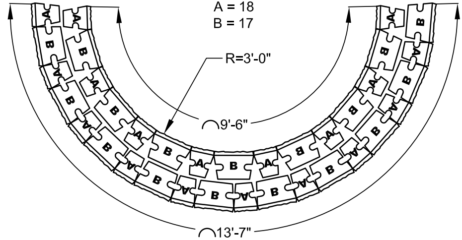
DS CAST STONE WALL 3 FT RADIUS DETAIL
