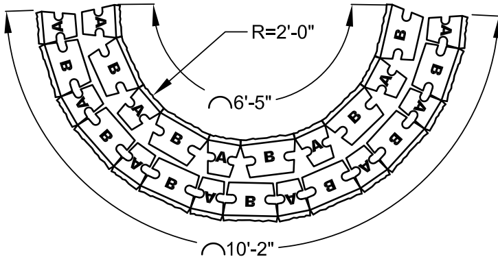
DS CAST STONE WALL 2 FT RADIUS DETAIL
