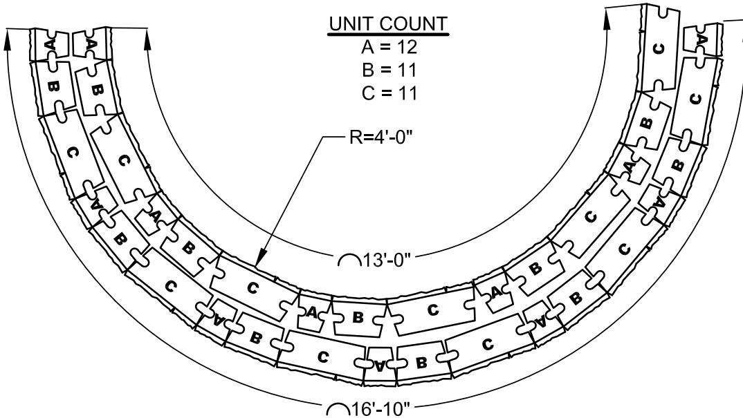
DS CAST STONE WALL 4 FT RADIUS DETAIL
