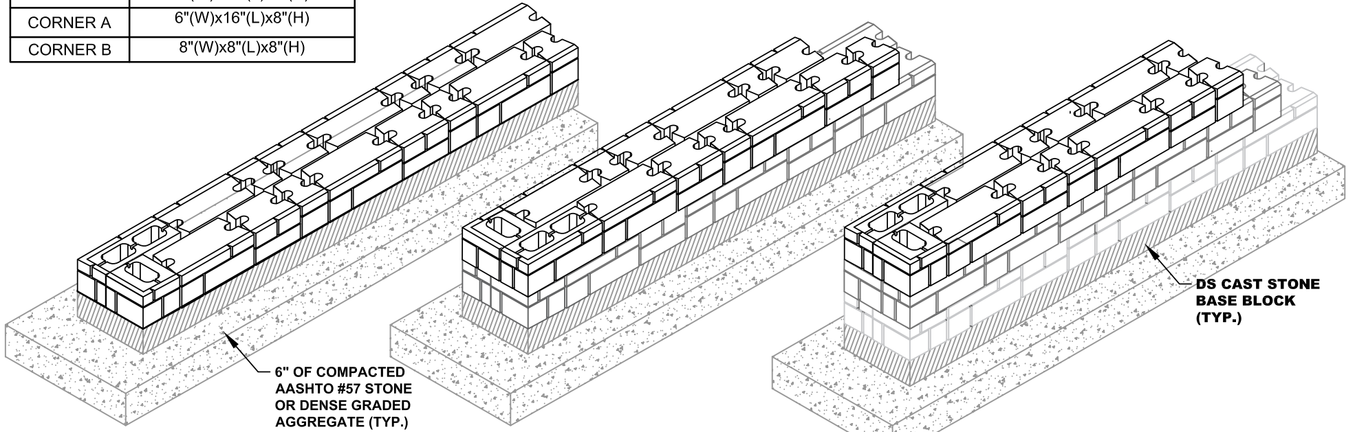
COURSE 1 PATTERN ISOMETRIC VIEW
