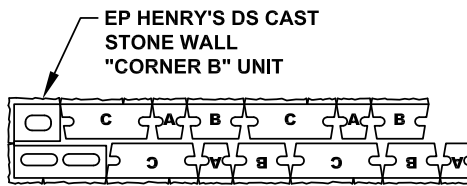
COURSE 2 PATTERN PLAN VIEW
