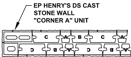
COURSE 1 PATTERN PLAN VIEW
