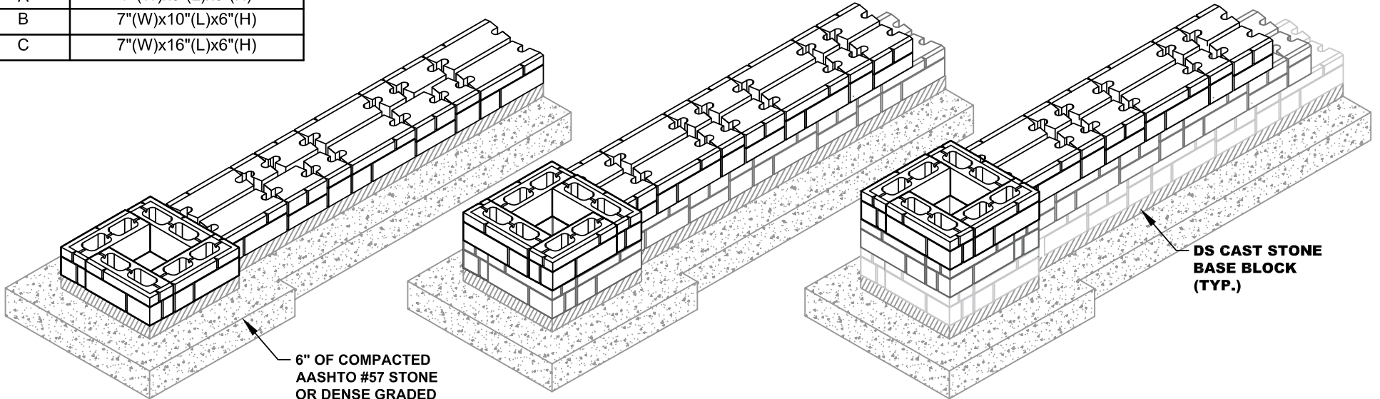
COURSE 1 PATTERN ISOMETRIC VIEW
