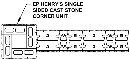
COURSE 1 PATTERN PLAN VIEW
