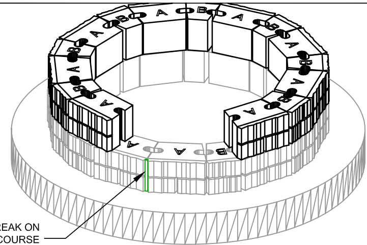
CONSTRUCTION SEQUENCE COURSE 2
