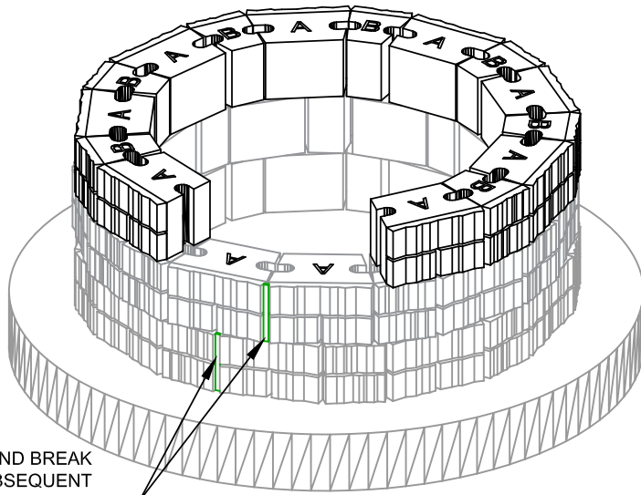
CONSTRUCTION SEQUENCE COURSE 3
