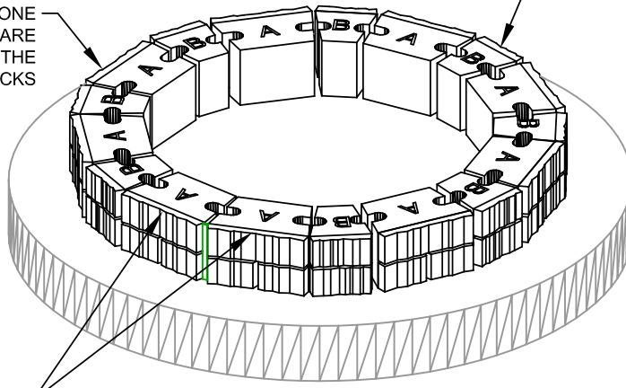
CONSTRUCTION SEQUENCE COURSE 1
