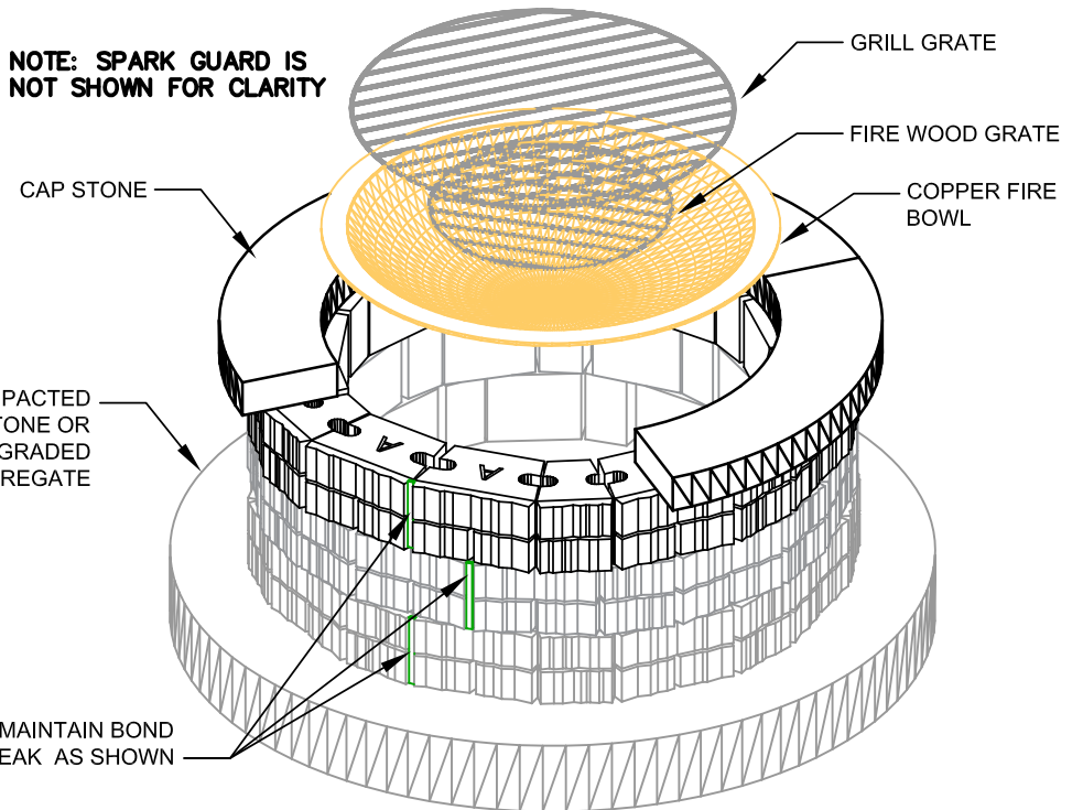
CAST STONE WALL FIRE PIT WITH GRILL ACCESSORIES
