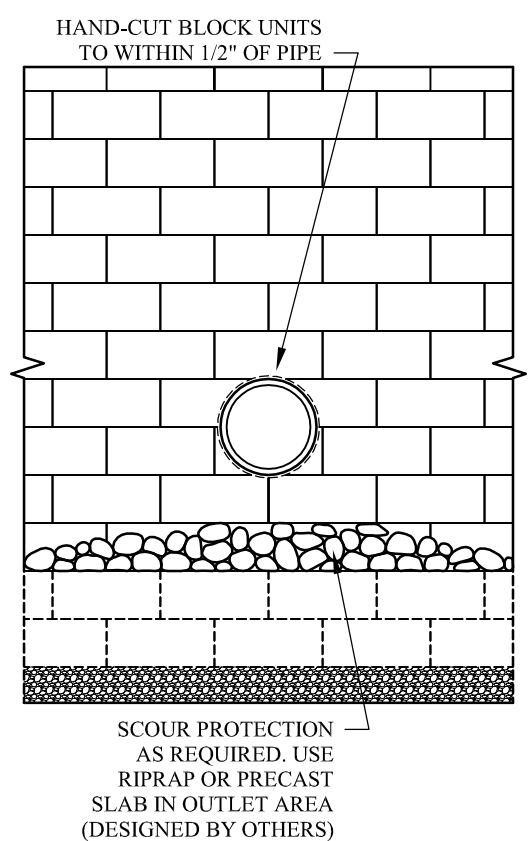
ELEVATION VIEW
