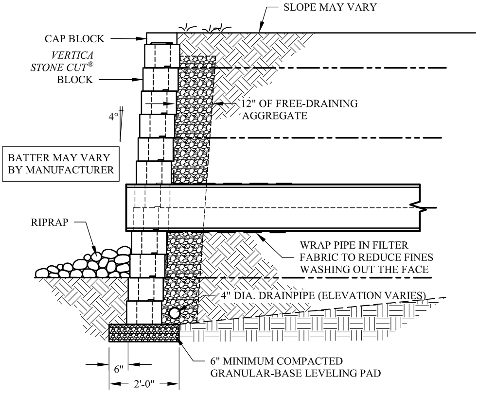
SECTION VIEW
