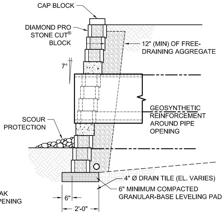
SECTION VIEW
