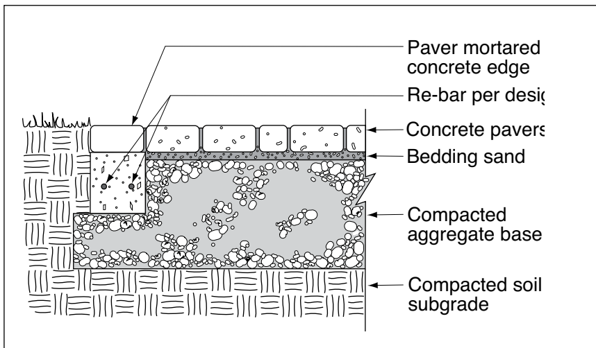
Figure 9. Submerged concrete edge.
