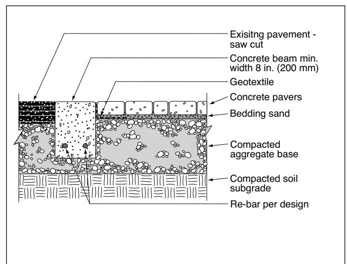
Figure 13. Crosswalk in existing asphalt pavement.
