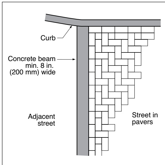
Figure 11. Concrete beam.
