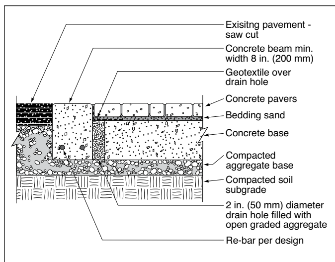
Figure 12. Crosswalk with concrete base.
