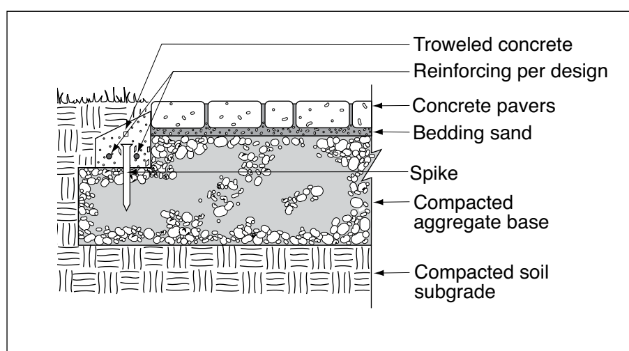
Figure 8. Troweled reinforced mortar edges.
