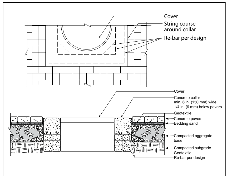
Figure 10. Utility cover.
