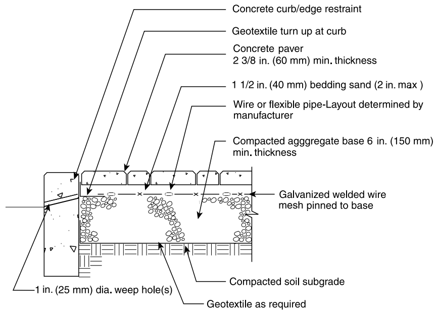
Heated sidewalk/residential driveway on compacted aggregate base
